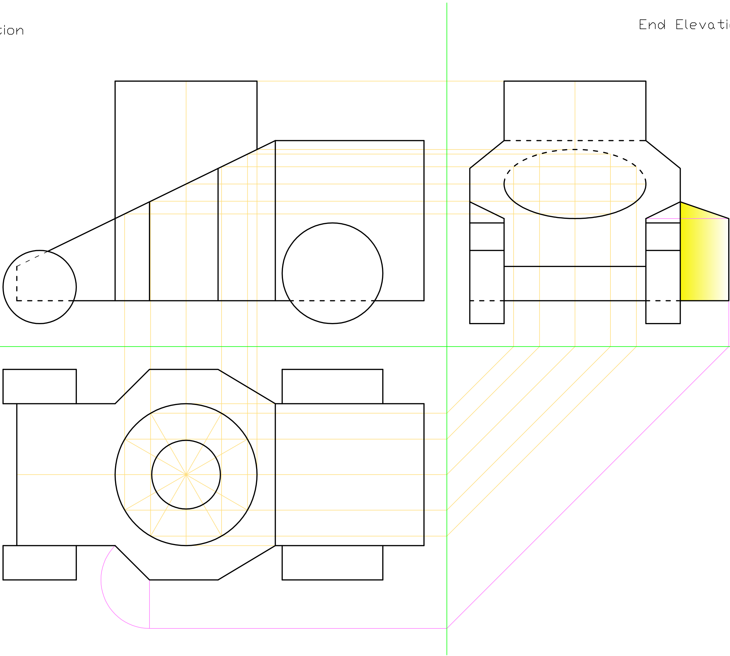
True Shape of Surface S
