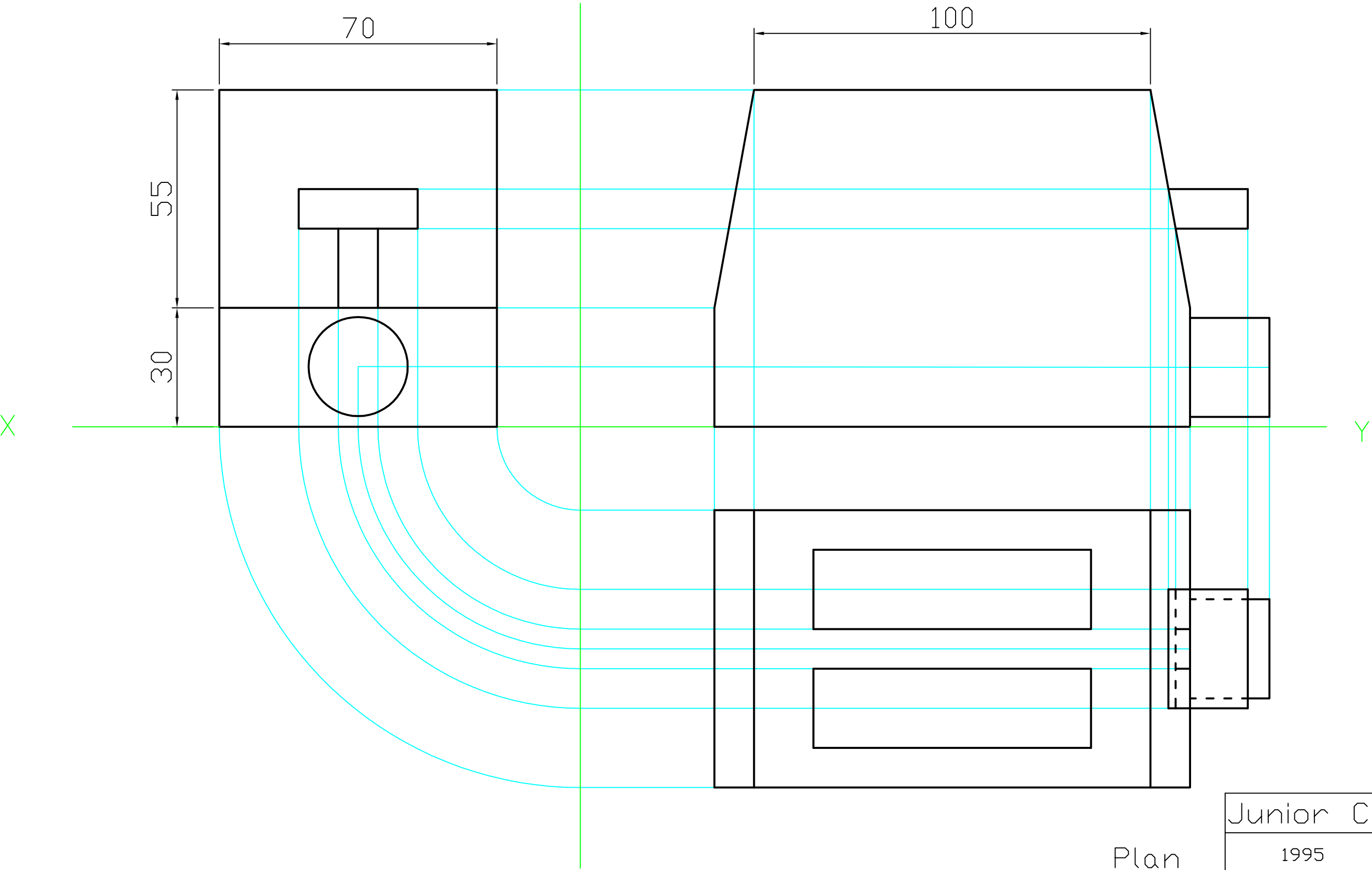
Front Elevation
