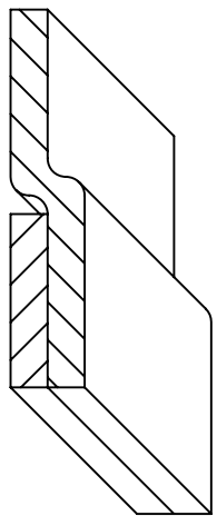
Soldered Lap Joint
