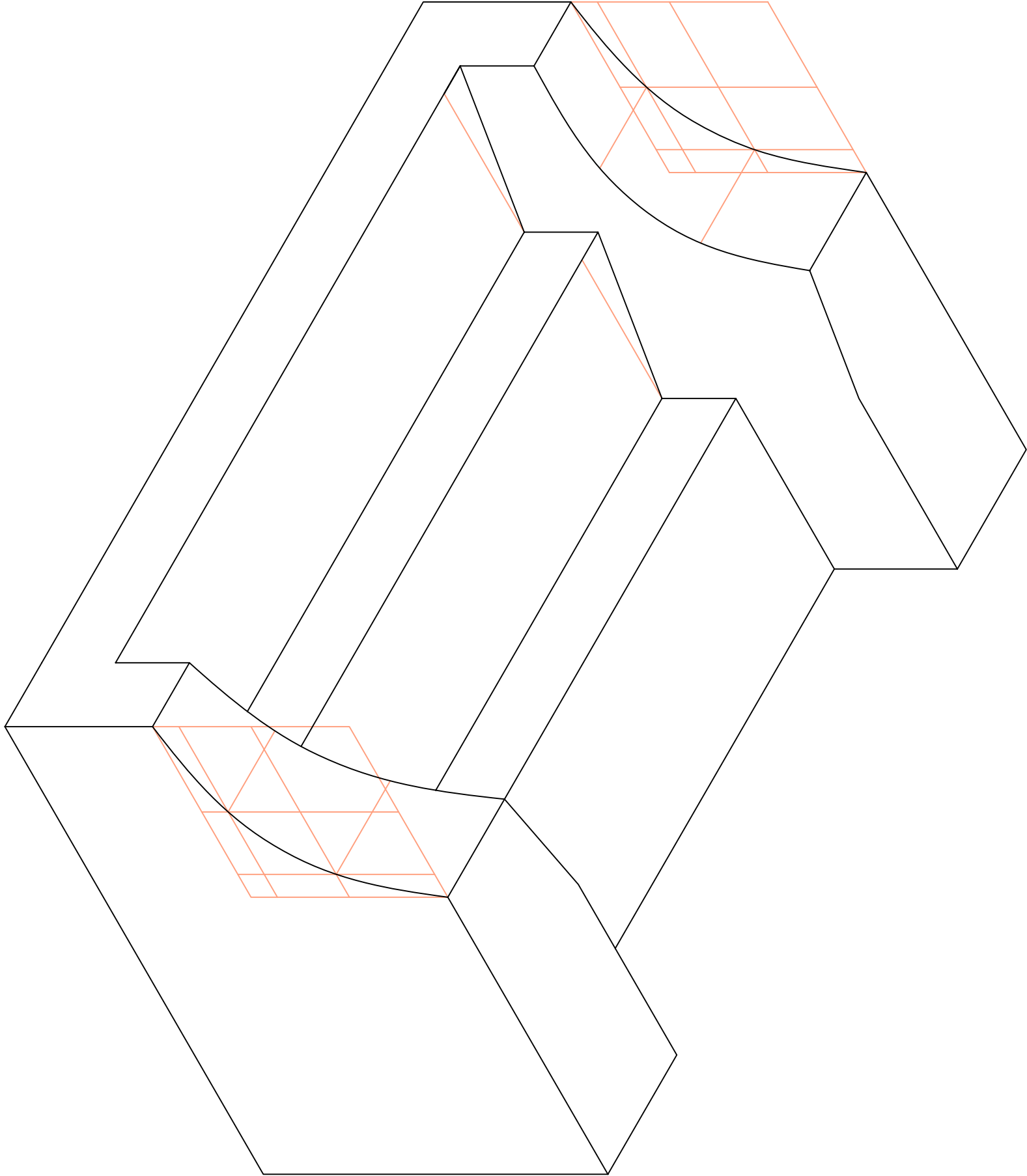
Isometric View
